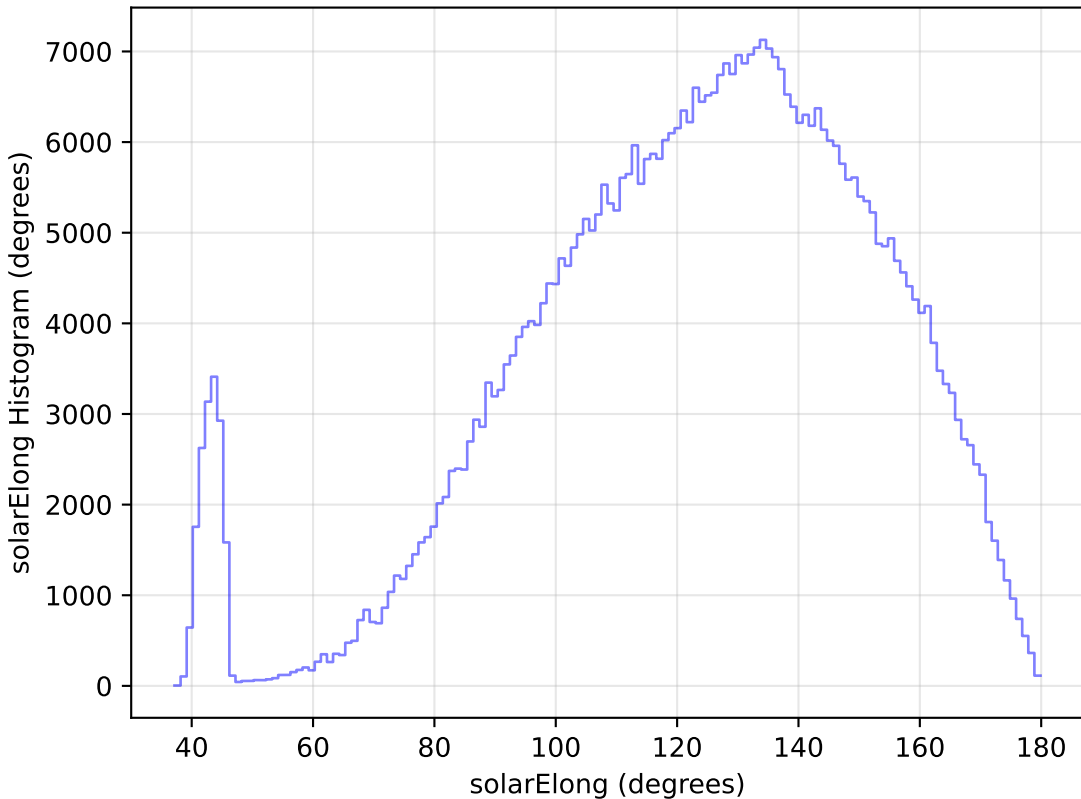
too_10_4v3.4_10yrs WFD r band: solarElong Histogram
