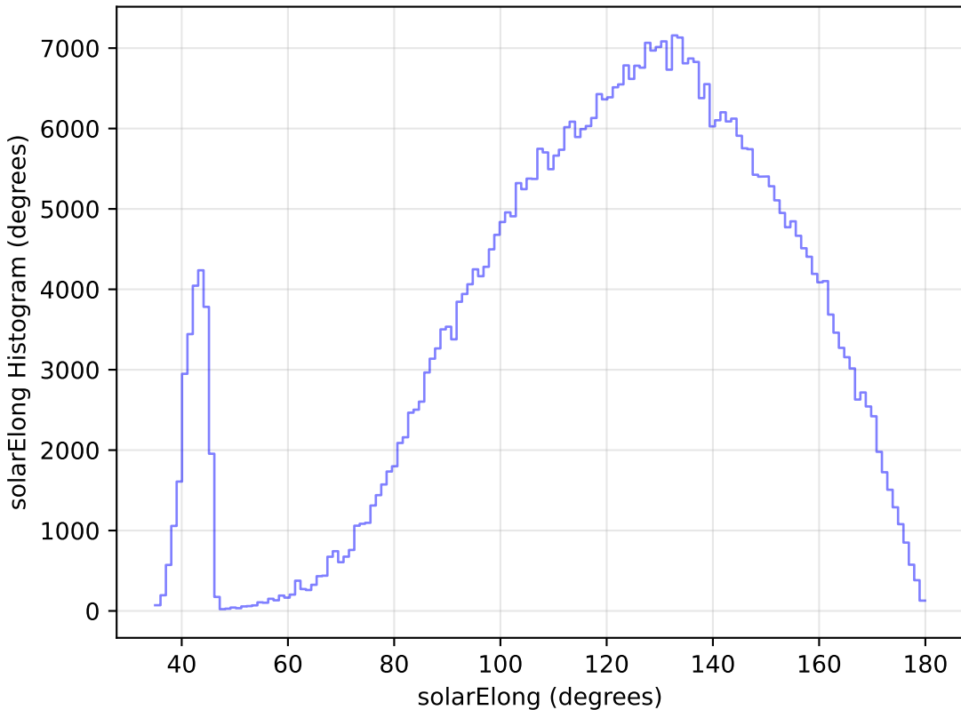
too_10_4v3.4_10yrs WFD i band: solarElong Histogram
