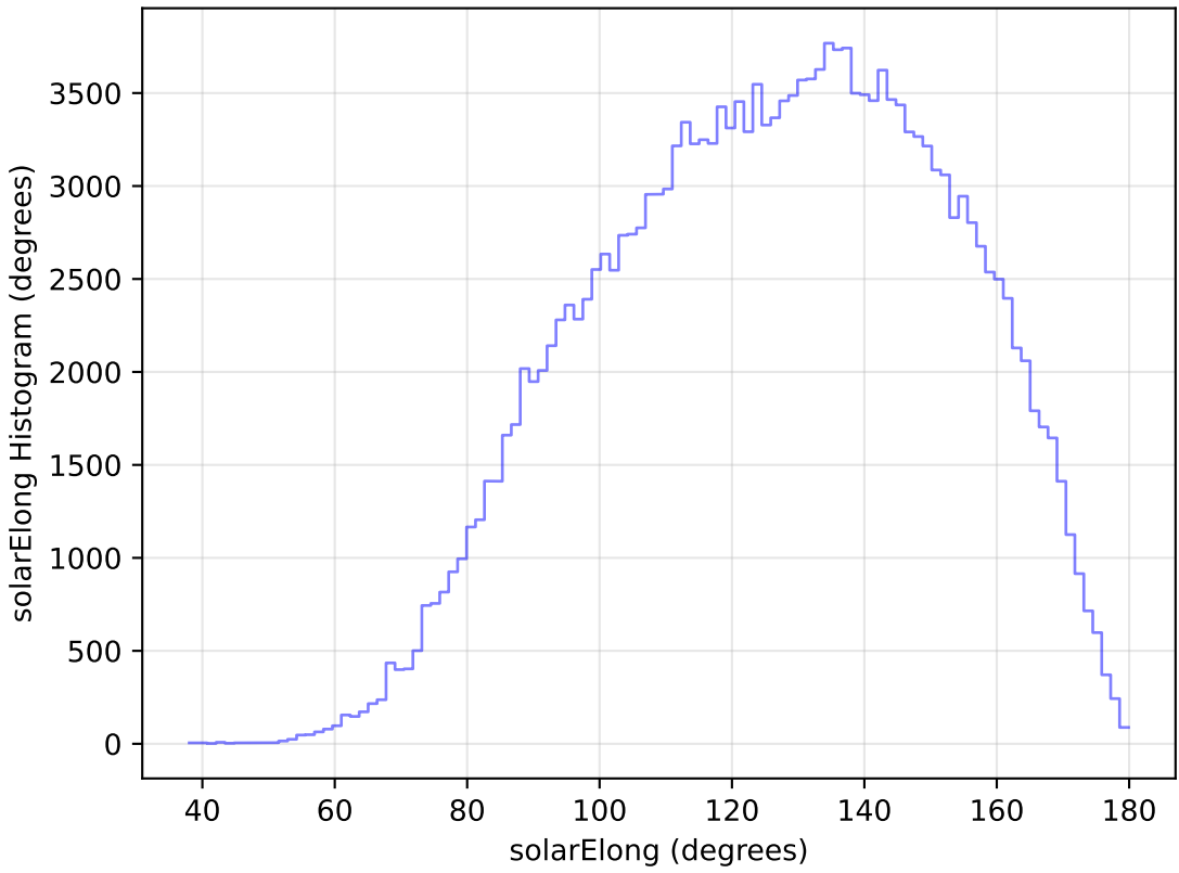
too_10_4v3.4_10yrs WFD g band: solarElong Histogram
