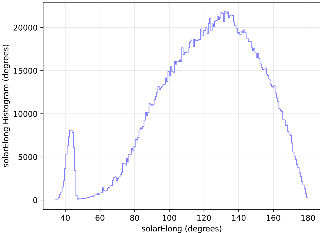
too_10_4v3.4_10yrs WFD all bands: solarElong Histogram
