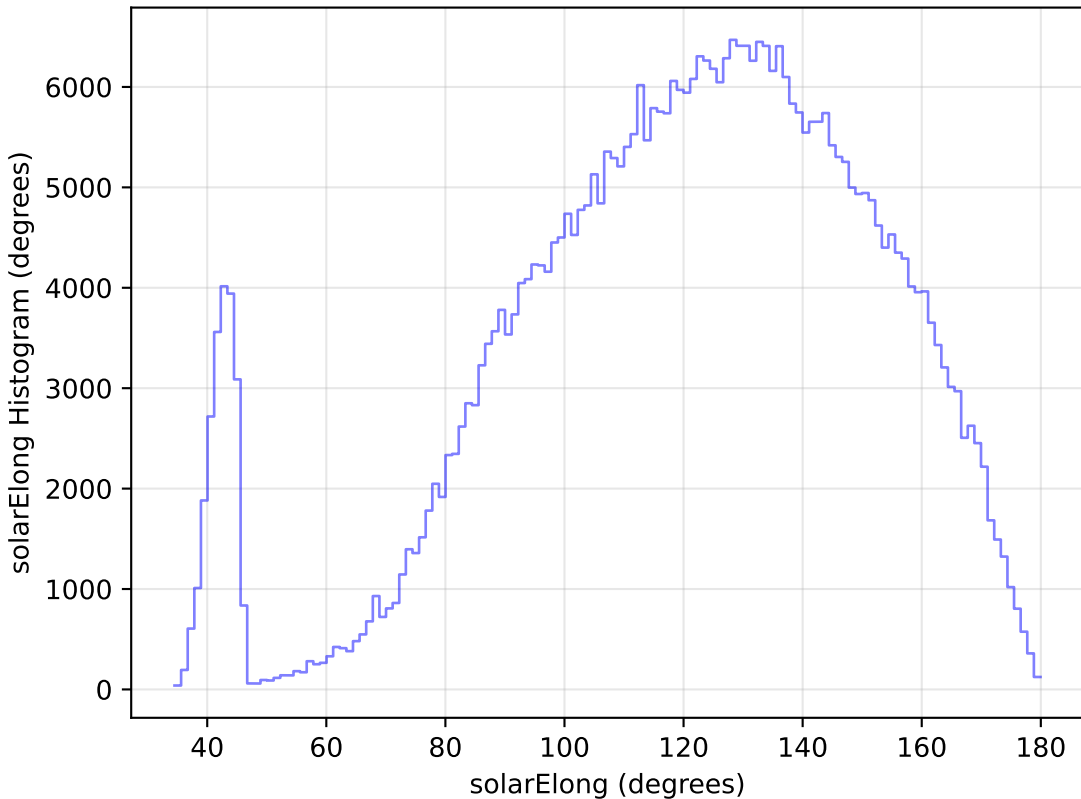
too_10_4v3.4_10yrs All sky z band: solarElong Histogram
