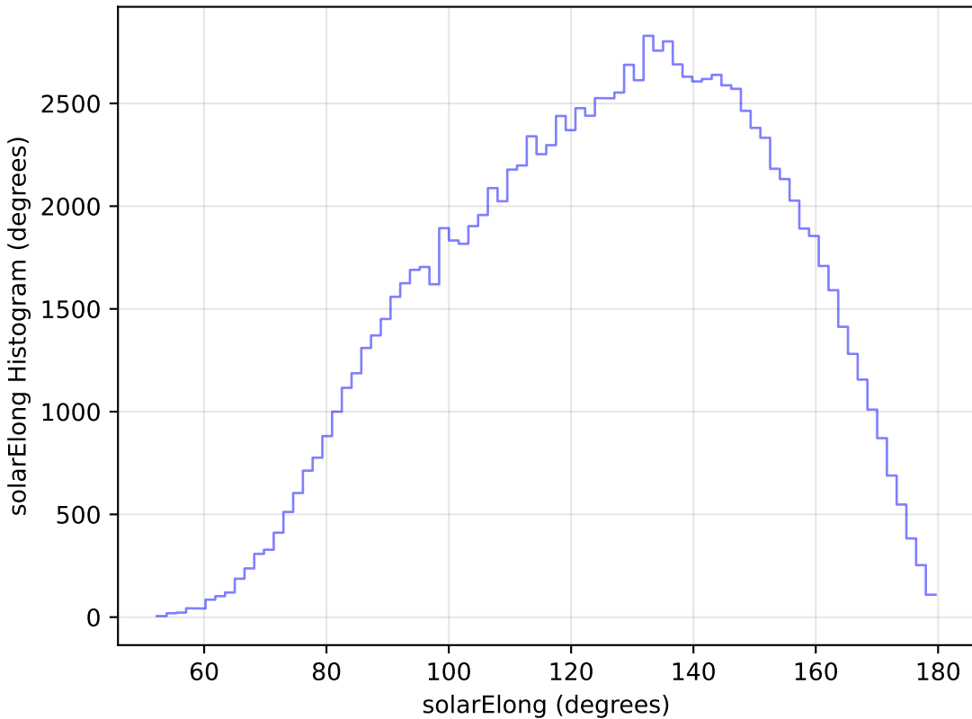
too_10_4v3.4_10yrs All sky u band: solarElong Histogram
