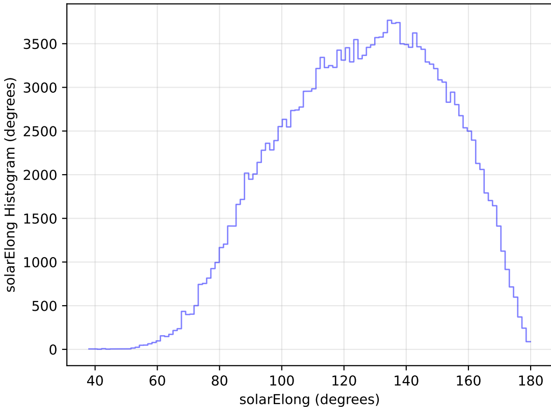
too_10_4v3.4_10yrs All sky g band: solarElong Histogram
