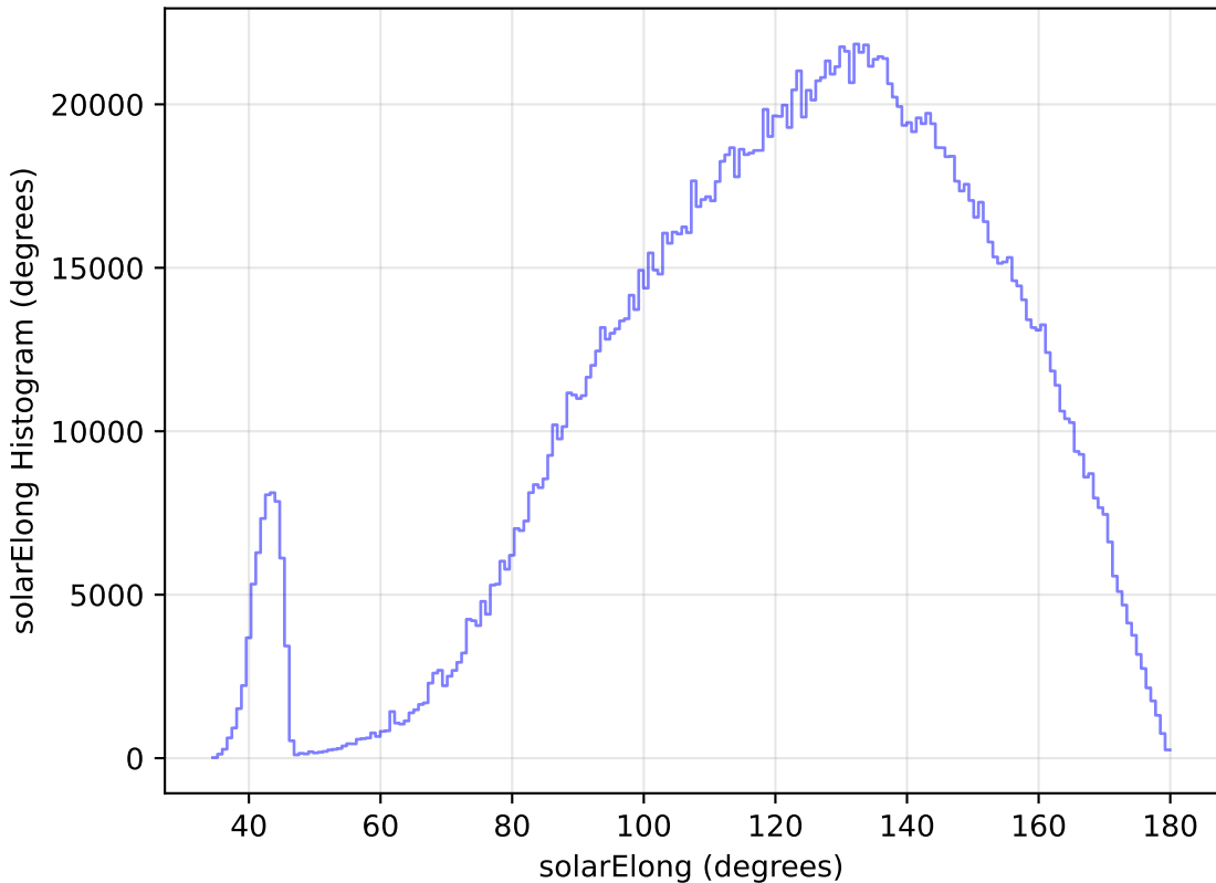
too_10_4v3.4_10yrs All sky all bands: solarElong Histogram
