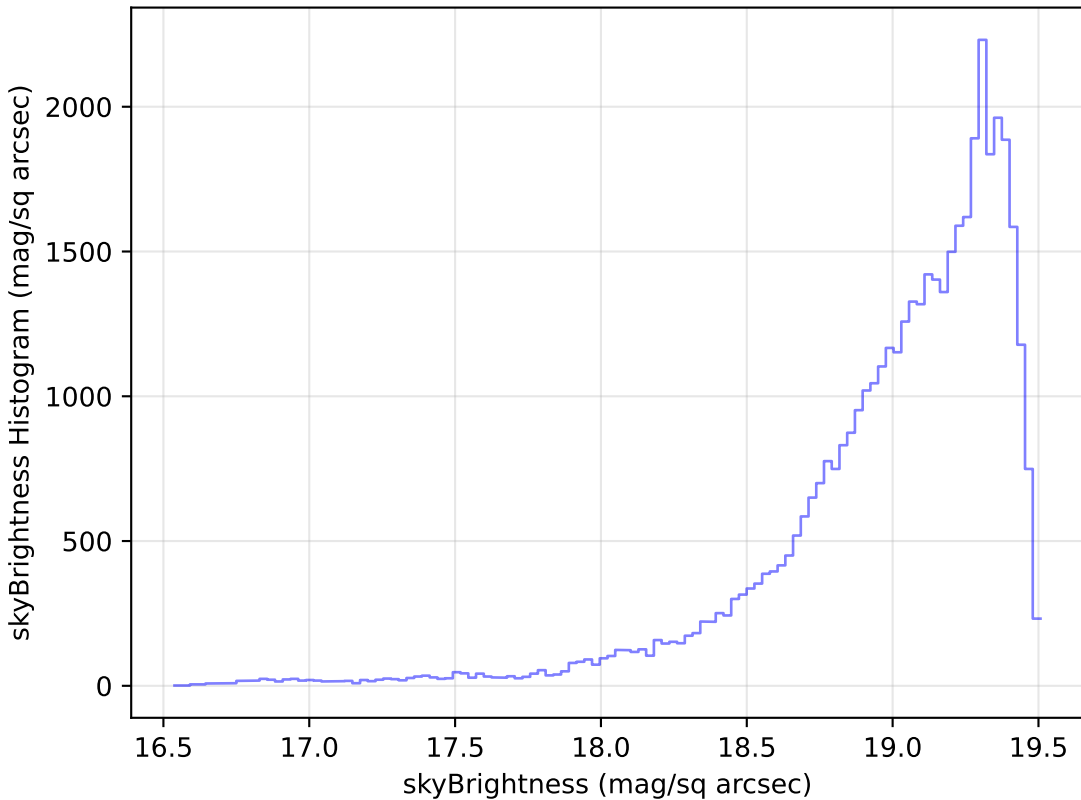
too_10_4v3.4_10yrs Yr 1 z band: skyBrightness Histogram
