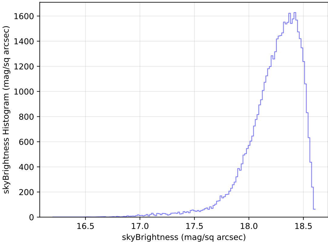
too_10_4v3.4_10yrs Yr 1 y band: skyBrightness Histogram
