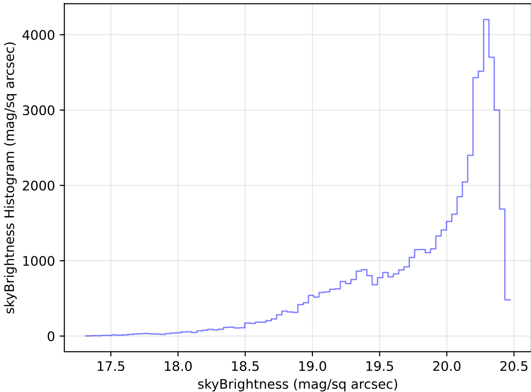
too_10_4v3.4_10yrs Yr 1 i band: skyBrightness Histogram
