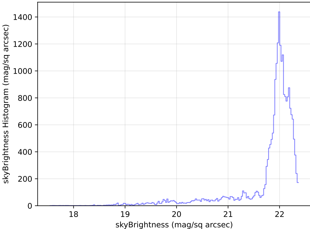
too_10_4v3.4_10yrs Yr 1 g band: skyBrightness Histogram
