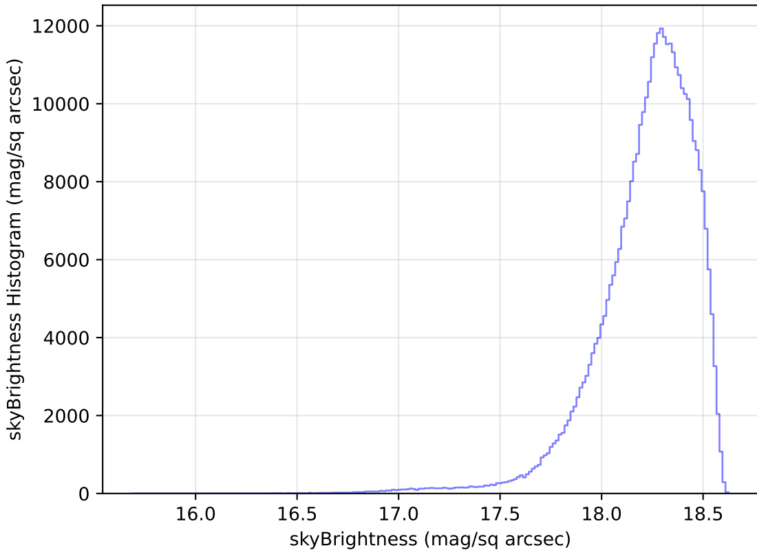
too_10_4v3.4_10yrs WFD y band: skyBrightness Histogram
