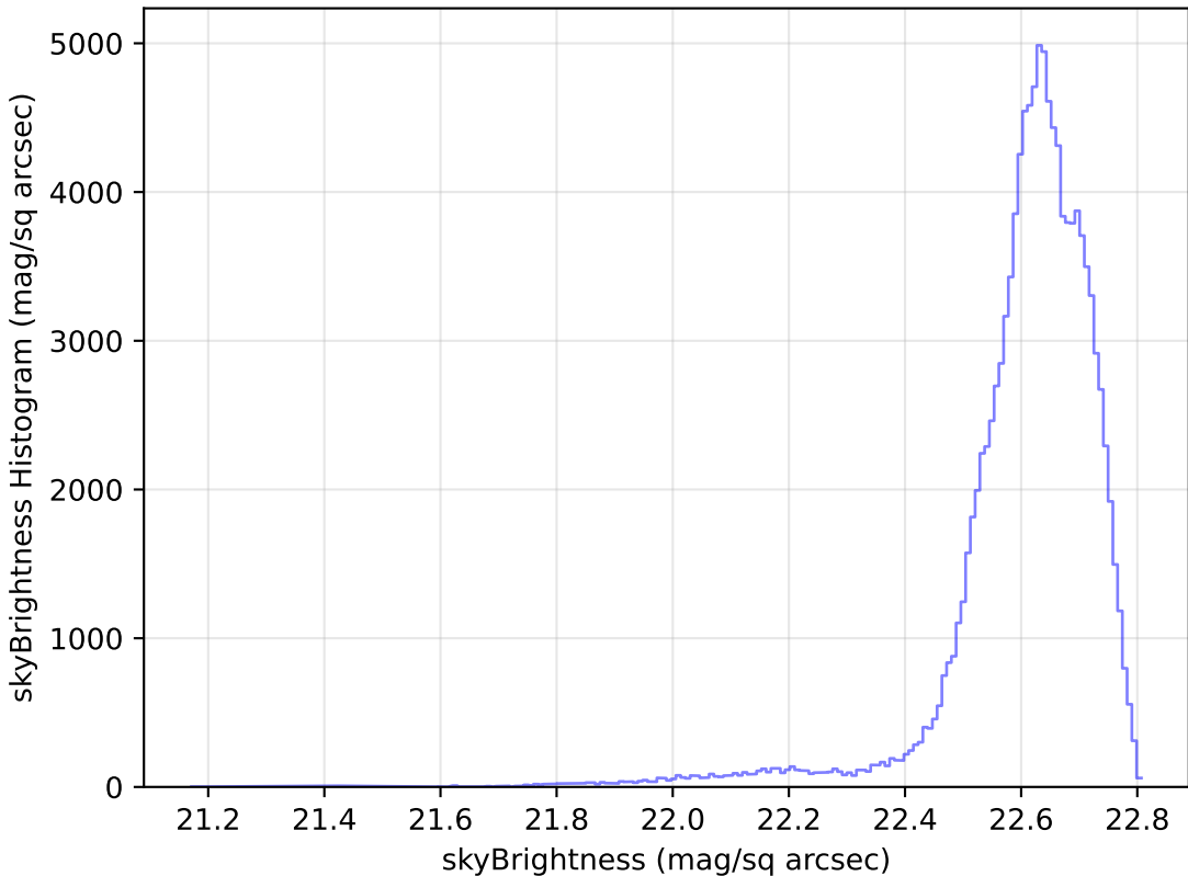
too_10_4v3.4_10yrs WFD u band: skyBrightness Histogram
