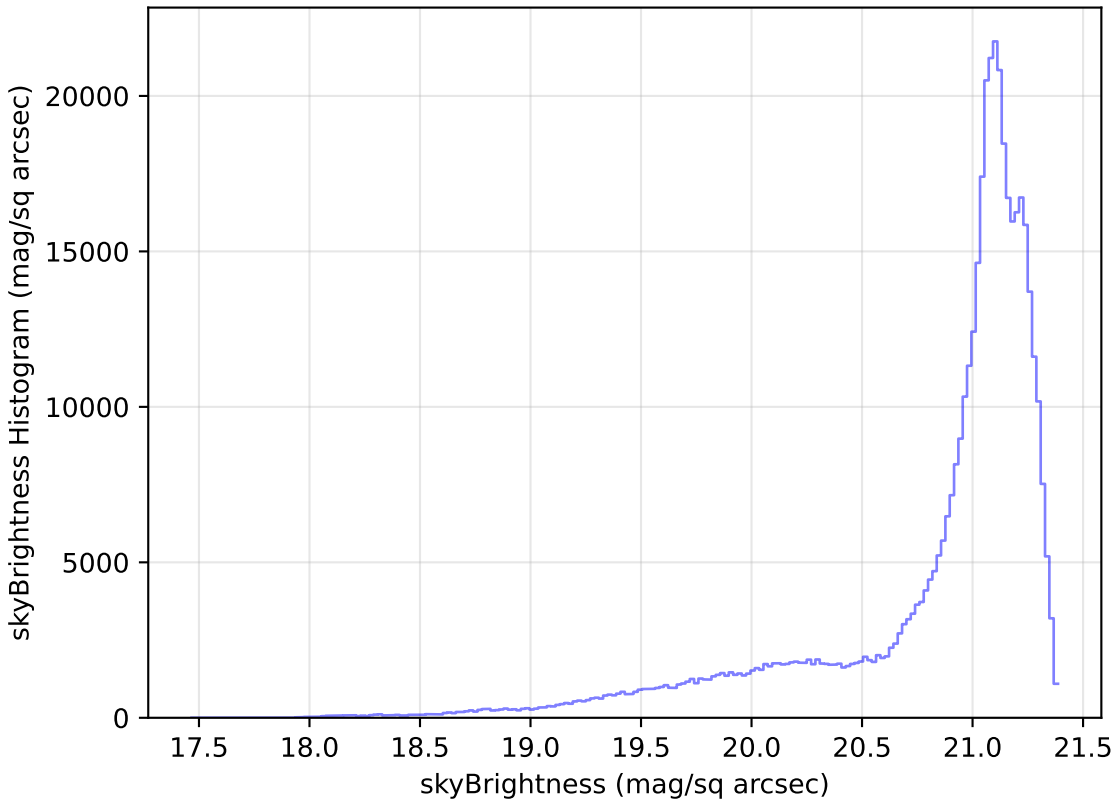
too_10_4v3.4_10yrs WFD r band: skyBrightness Histogram
