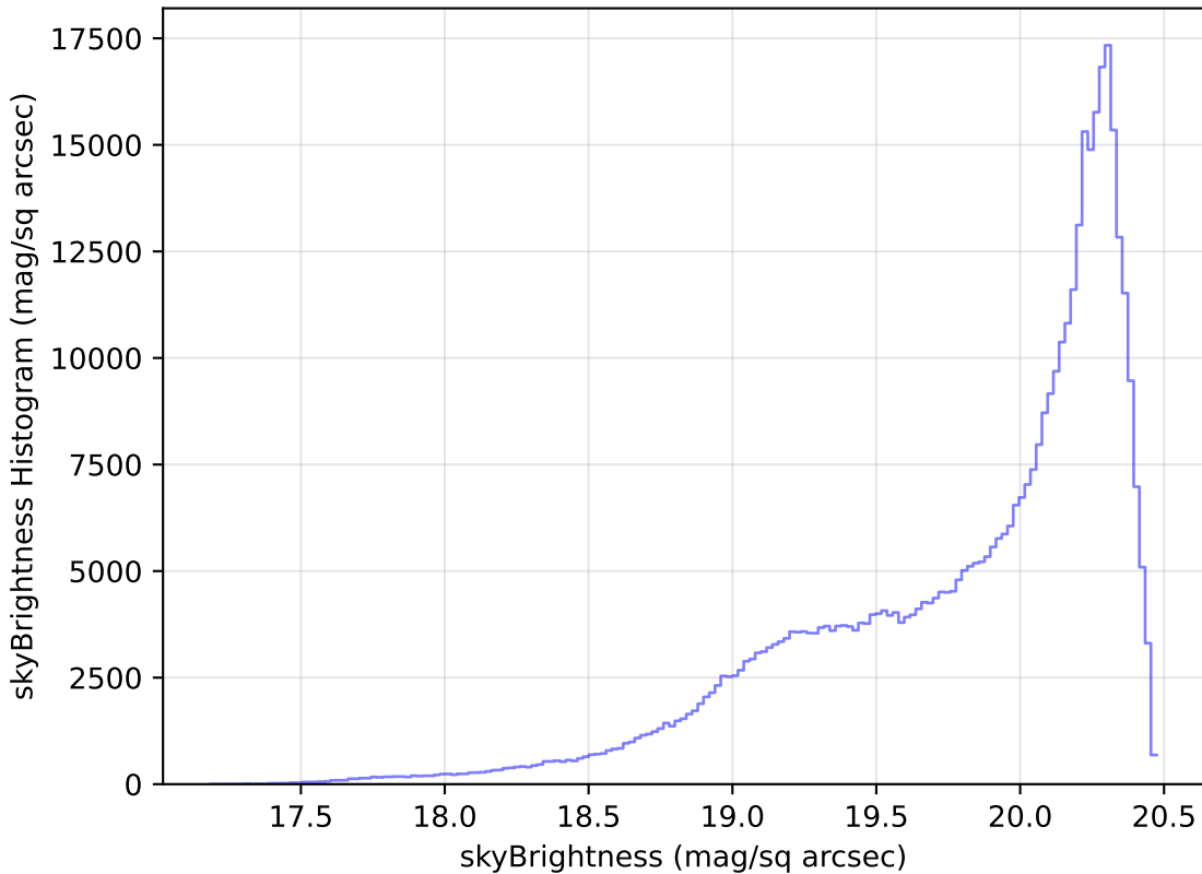
too_10_4v3.4_10yrs WFD i band: skyBrightness Histogram
