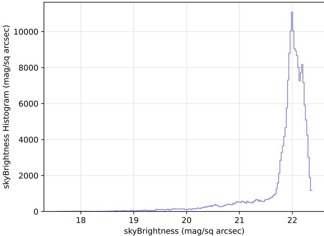
too_10_4v3.4_10yrs WFD g band: skyBrightness Histogram
