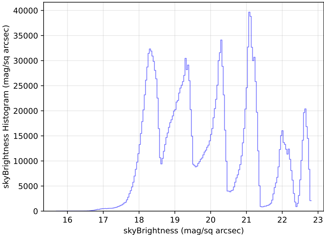
too_10_4v3.4_10yrs WFD all bands: skyBrightness Histogram
