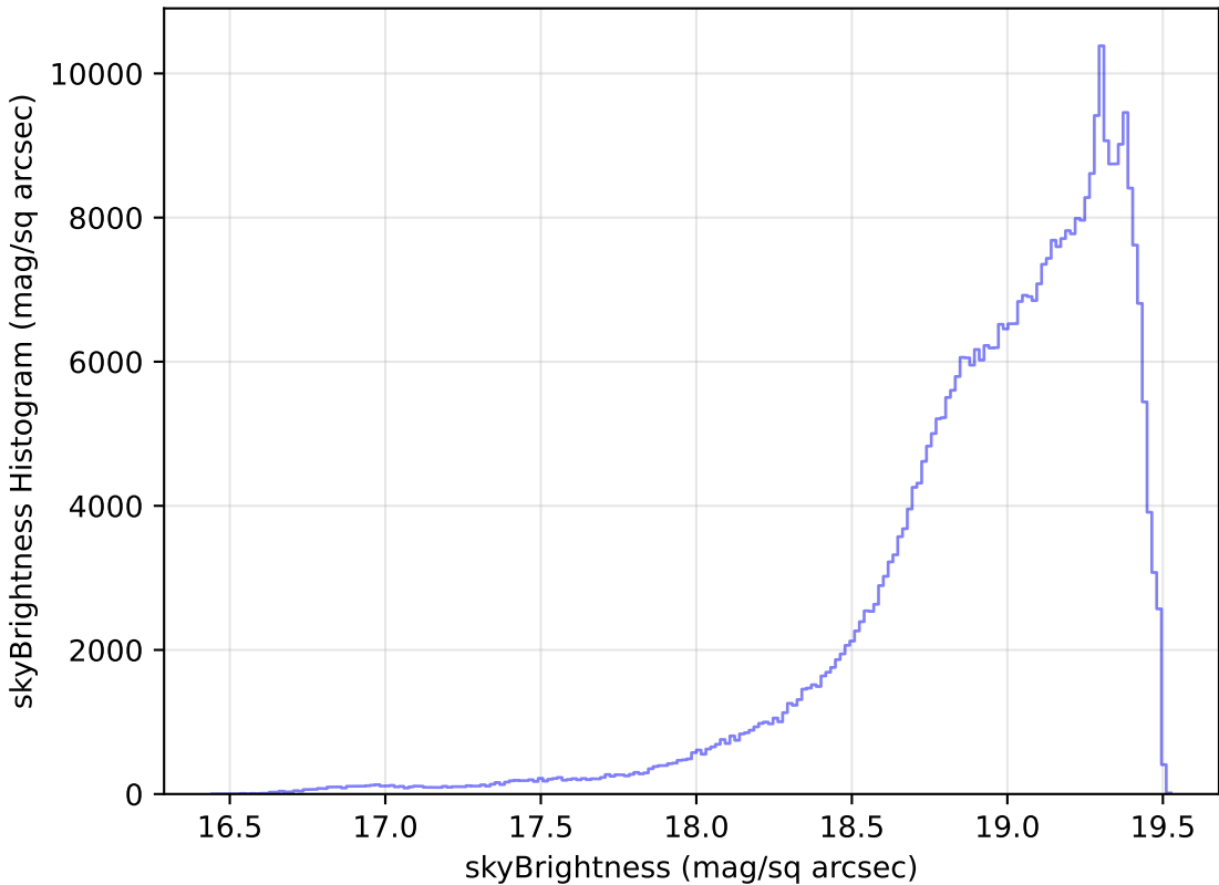
too_10_4v3.4_10yrs All sky z band: skyBrightness Histogram
