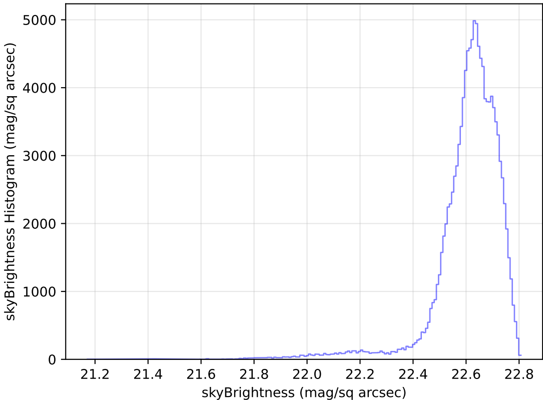
too_10_4v3.4_10yrs All sky u band: skyBrightness Histogram
