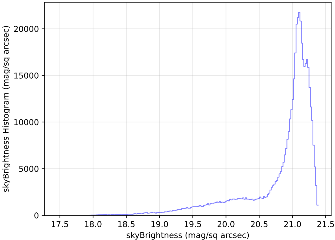
too_10_4v3.4_10yrs All sky r band: skyBrightness Histogram
