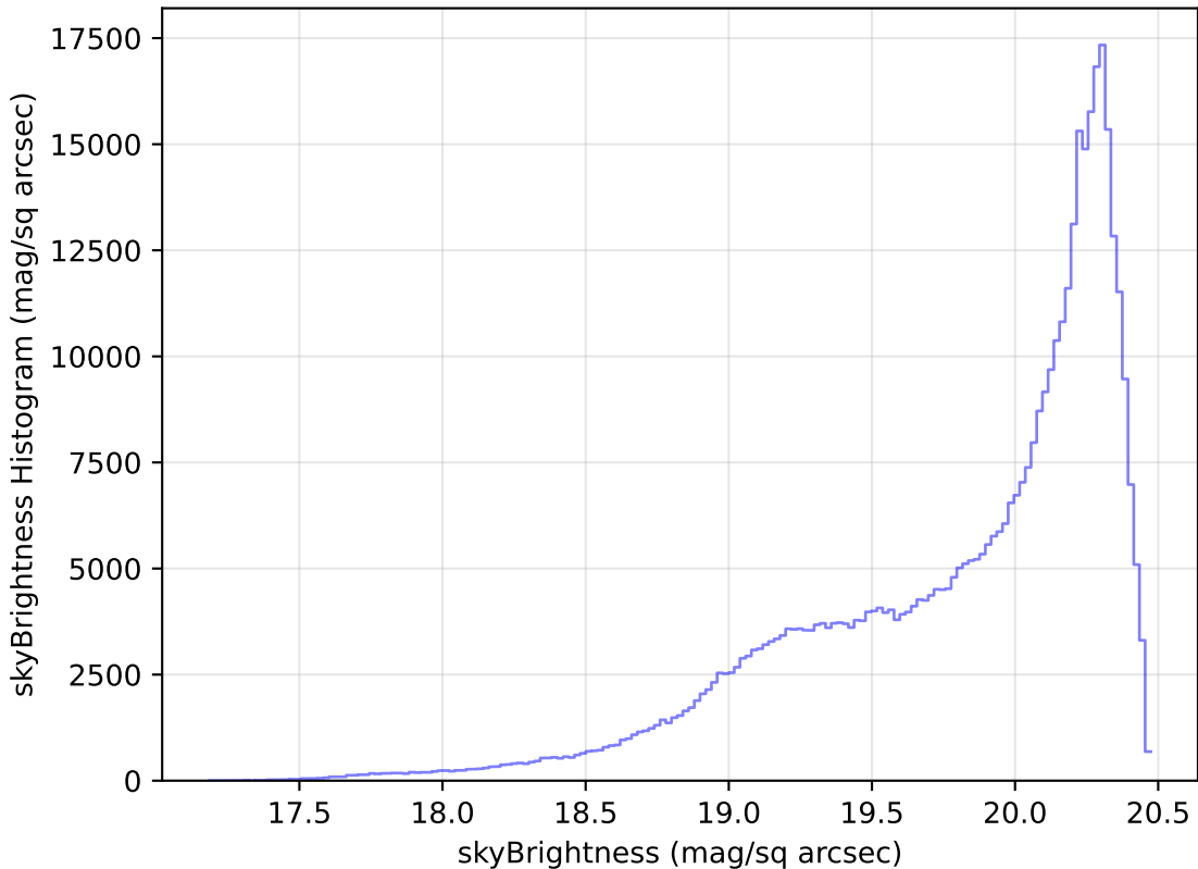
too_10_4v3.4_10yrs All sky i band: skyBrightness Histogram
