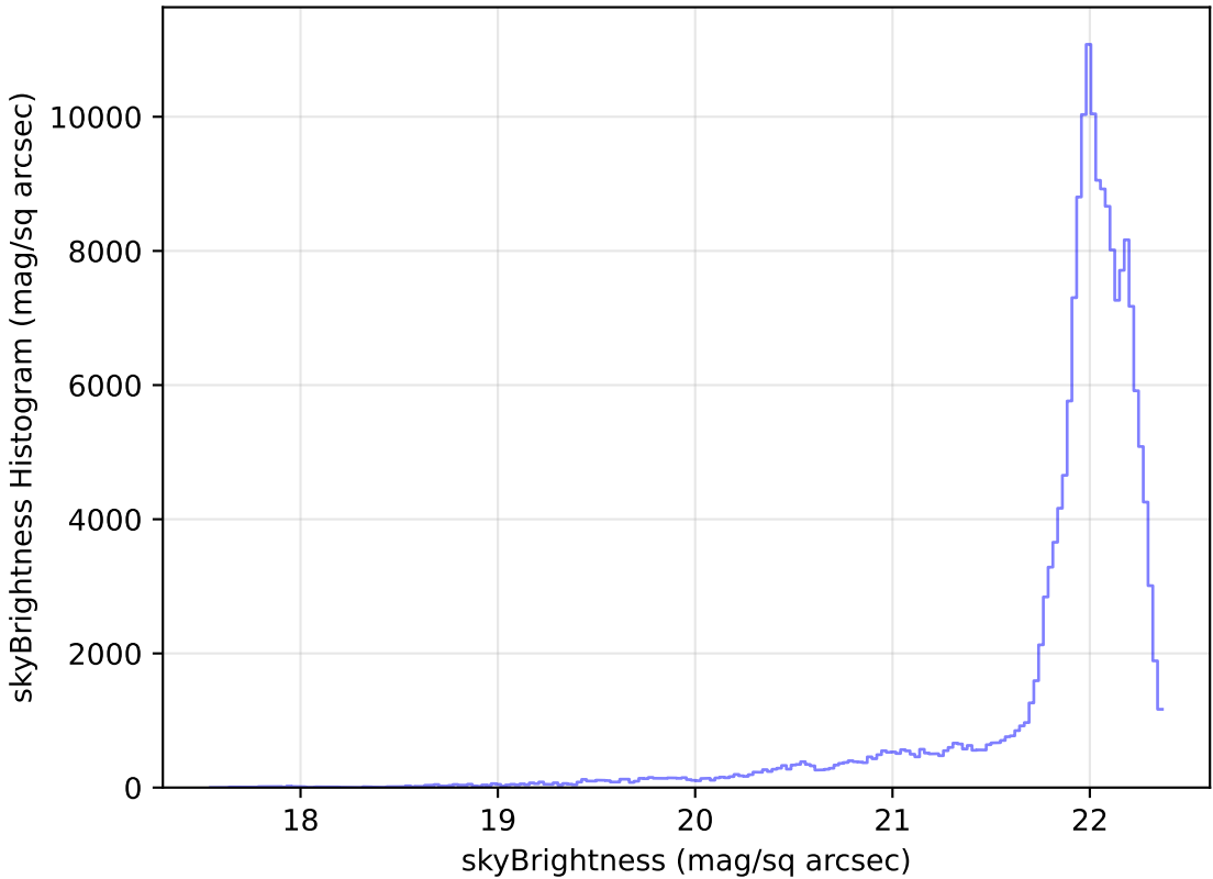
too_10_4v3.4_10yrs All sky g band: skyBrightness Histogram
