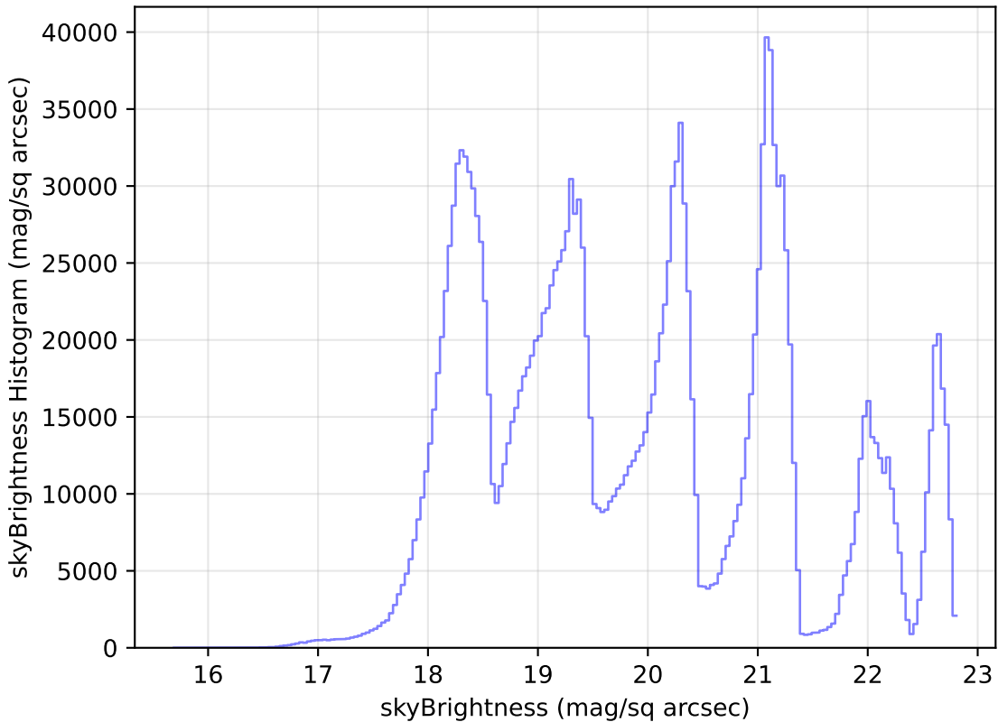
too_10_4v3.4_10yrs All sky all bands: skyBrightness Histogram
