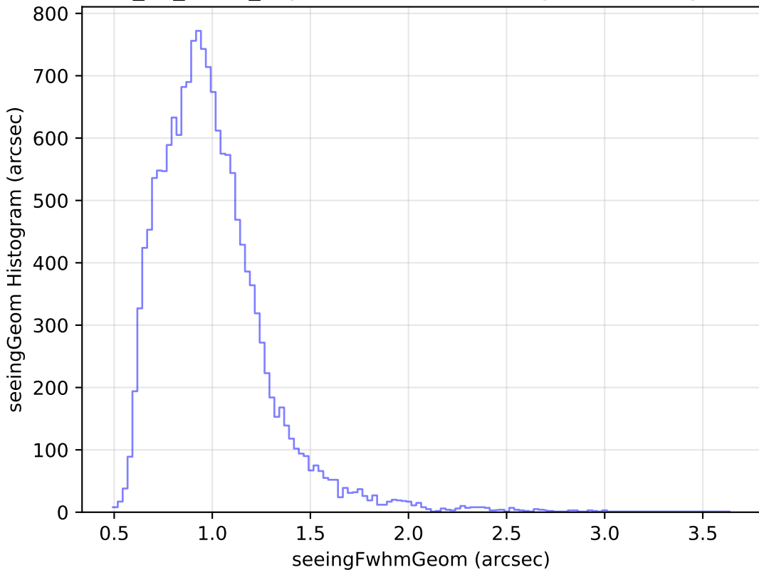
too_10_4v3.4_10yrs Yr 1 u band: seeingGeom Histogram
