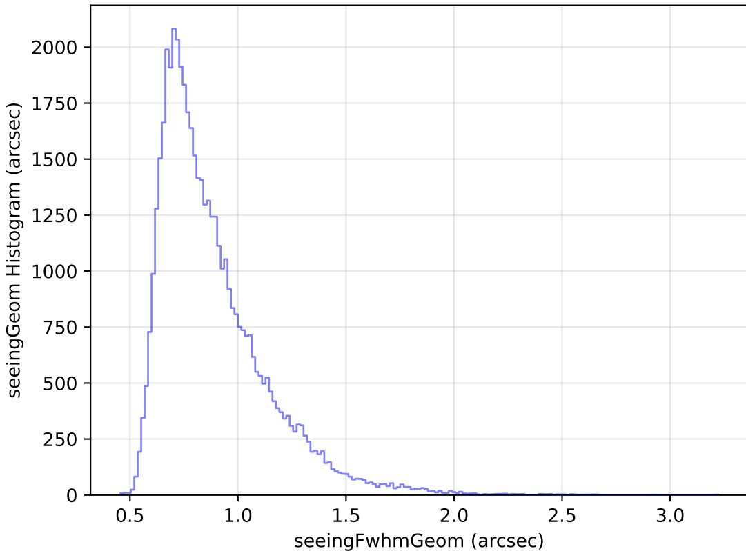
too_10_4v3.4_10yrs Yr 1 r band: seeingGeom Histogram
