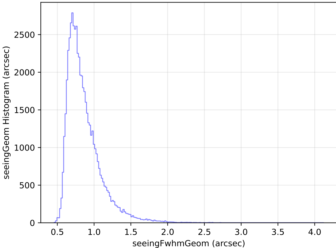
too_10_4v3.4_10yrs Yr 1 i band: seeingGeom Histogram
