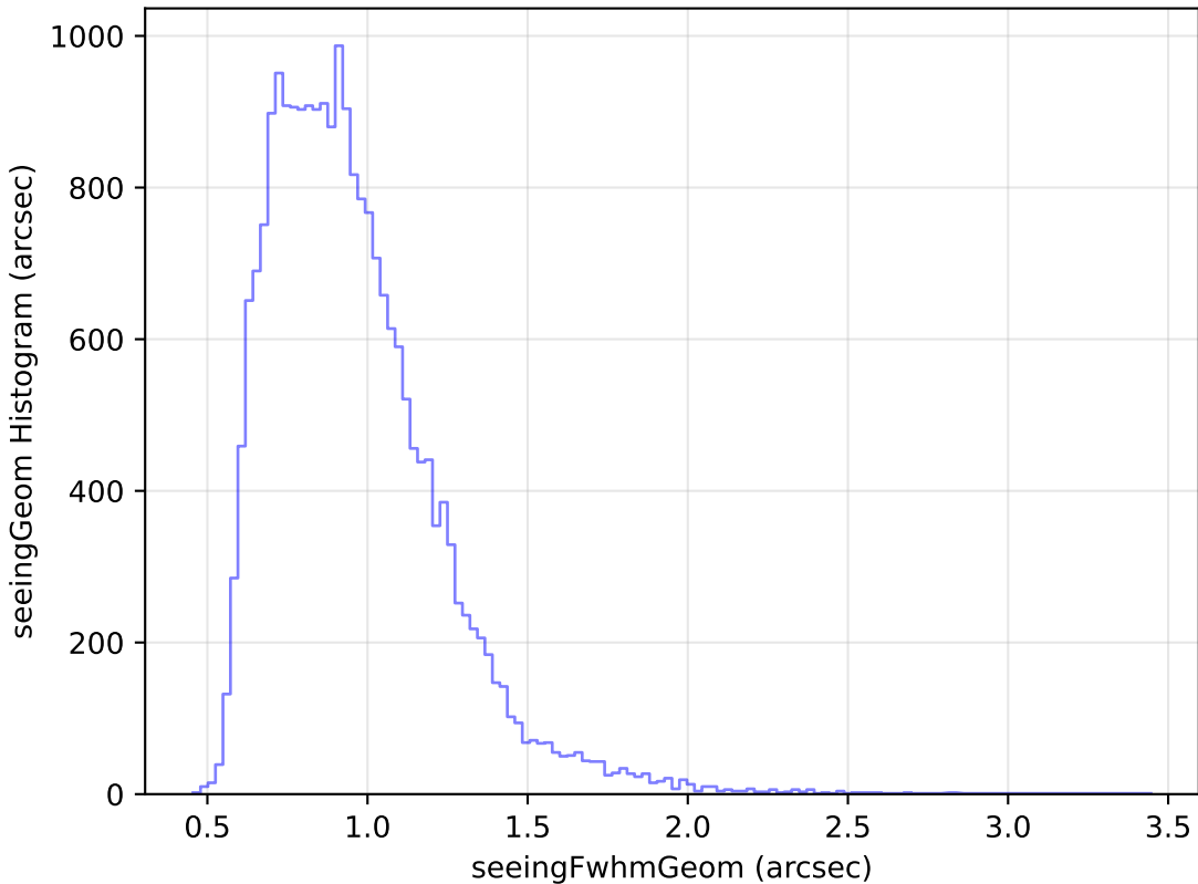
too_10_4v3.4_10yrs Yr 1 g band: seeingGeom Histogram
