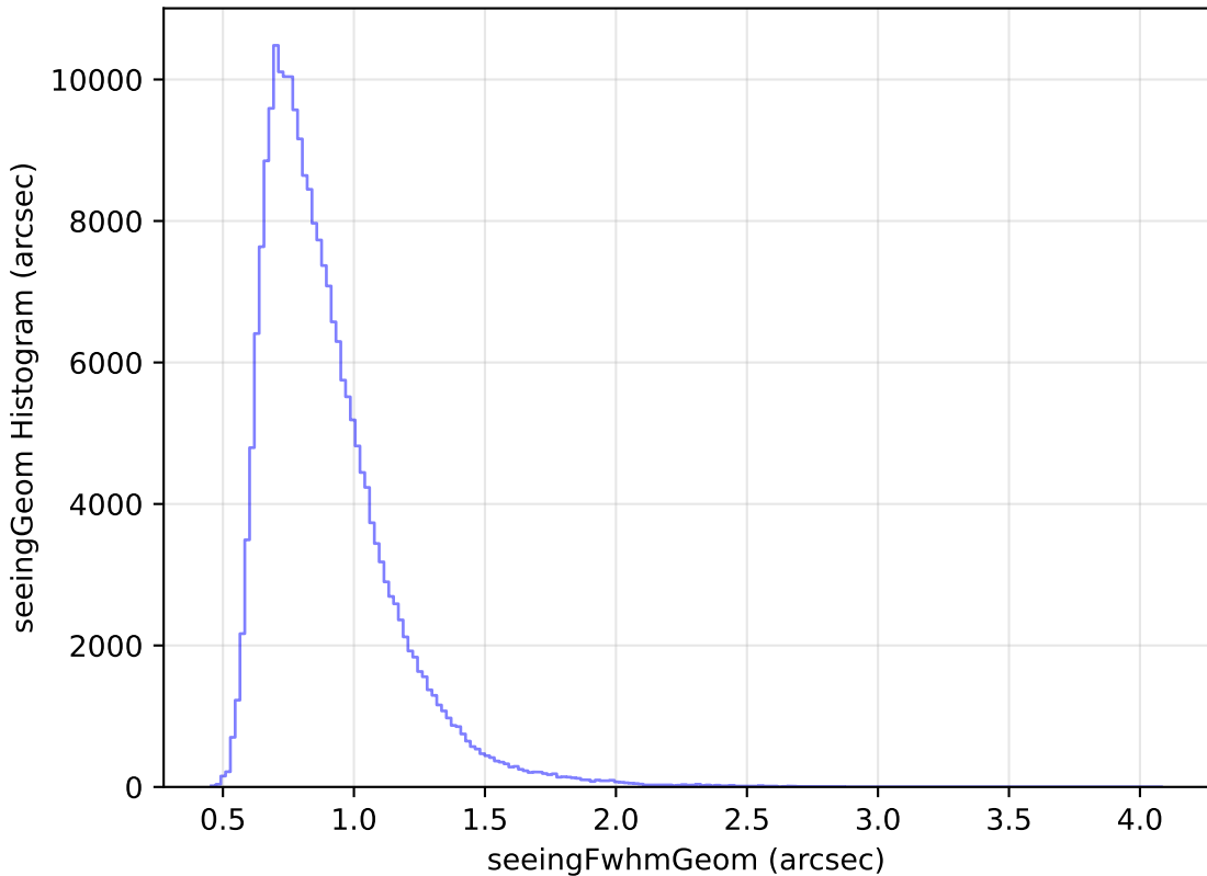
too_10_4v3.4_10yrs Yr 1 all bands: seeingGeom Histogram
