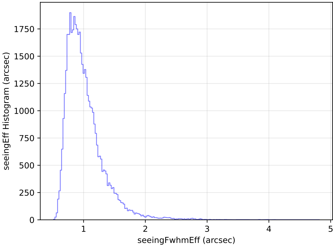
too_10_4v3.4_10yrs Yr 1 z band: seeingEff Histogram
