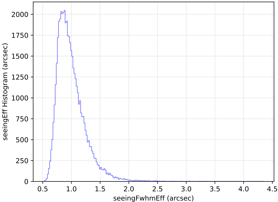
too_10_4v3.4_10yrs Yr 1 y band: seeingEff Histogram
