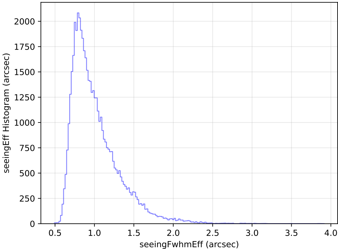
too_10_4v3.4_10yrs Yr 1 r band: seeingEff Histogram
