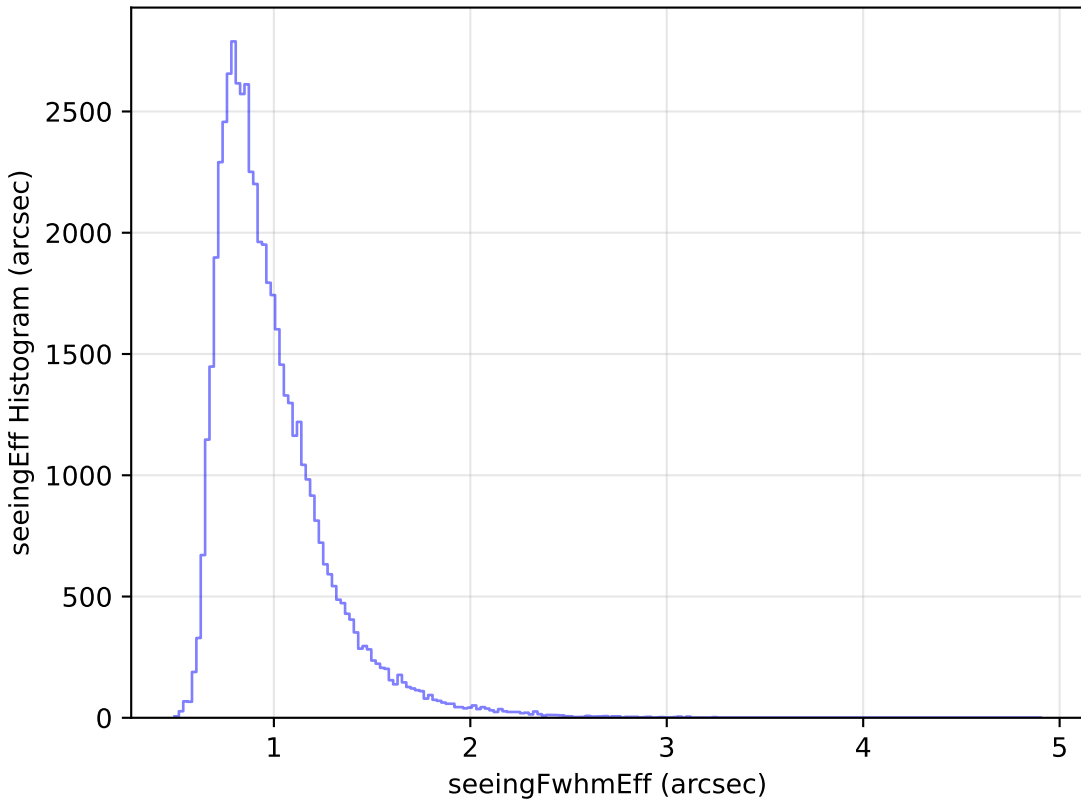
too_10_4v3.4_10yrs Yr 1 i band: seeingEff Histogram
