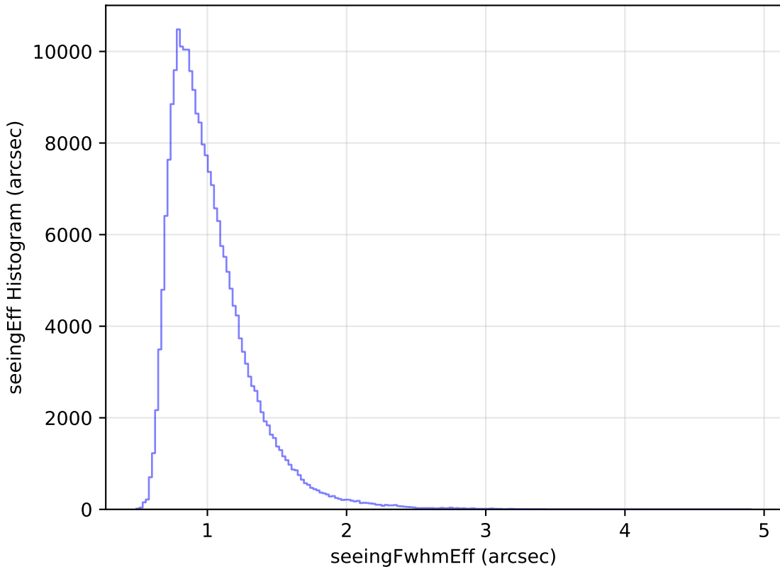
too_10_4v3.4_10yrs Yr 1 all bands: seeingEff Histogram
