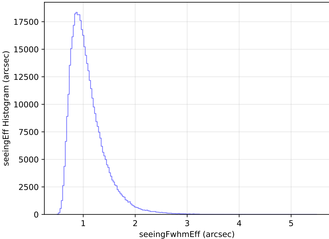
too_10_4v3.4_10yrs WFD z band: seeingEff Histogram
