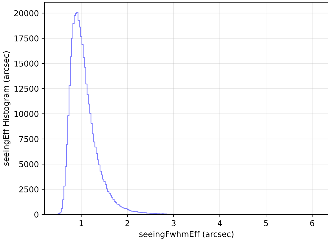
too_10_4v3.4_10yrs WFD y band: seeingEff Histogram
