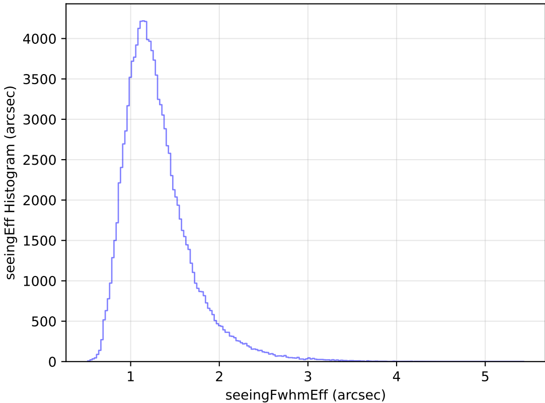
too_10_4v3.4_10yrs WFD u band: seeingEff Histogram
