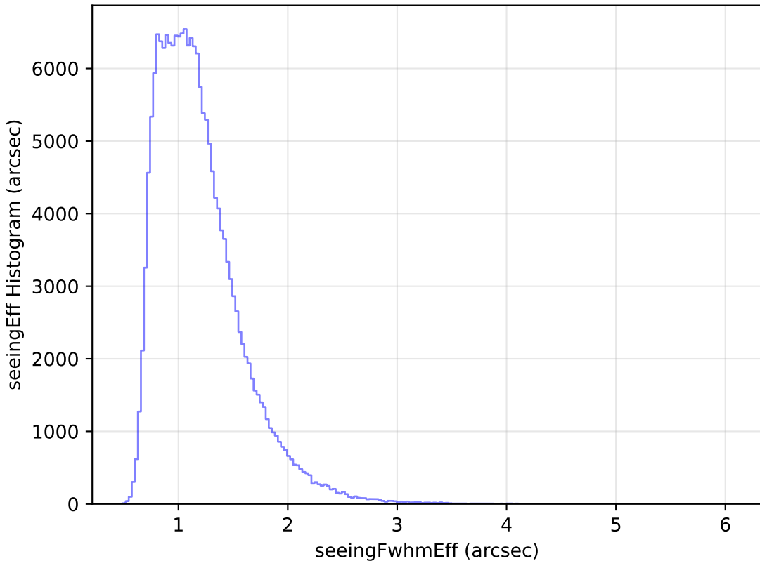
too_10_4v3.4_10yrs WFD g band: seeingEff Histogram
