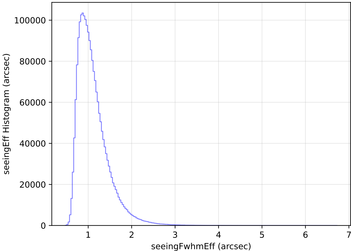
too_10_4v3.4_10yrs WFD all bands: seeingEff Histogram
