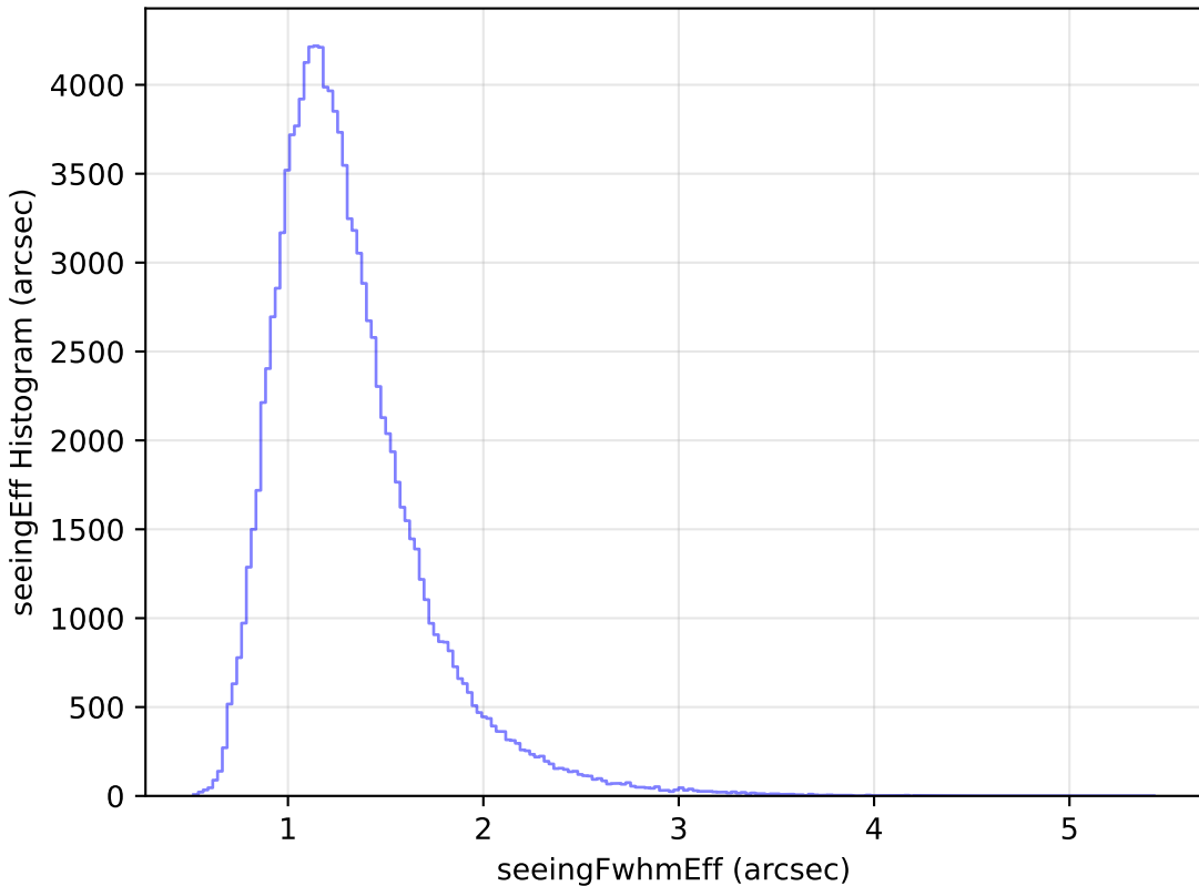
too_10_4v3.4_10yrs All sky u band: seeingEff Histogram
