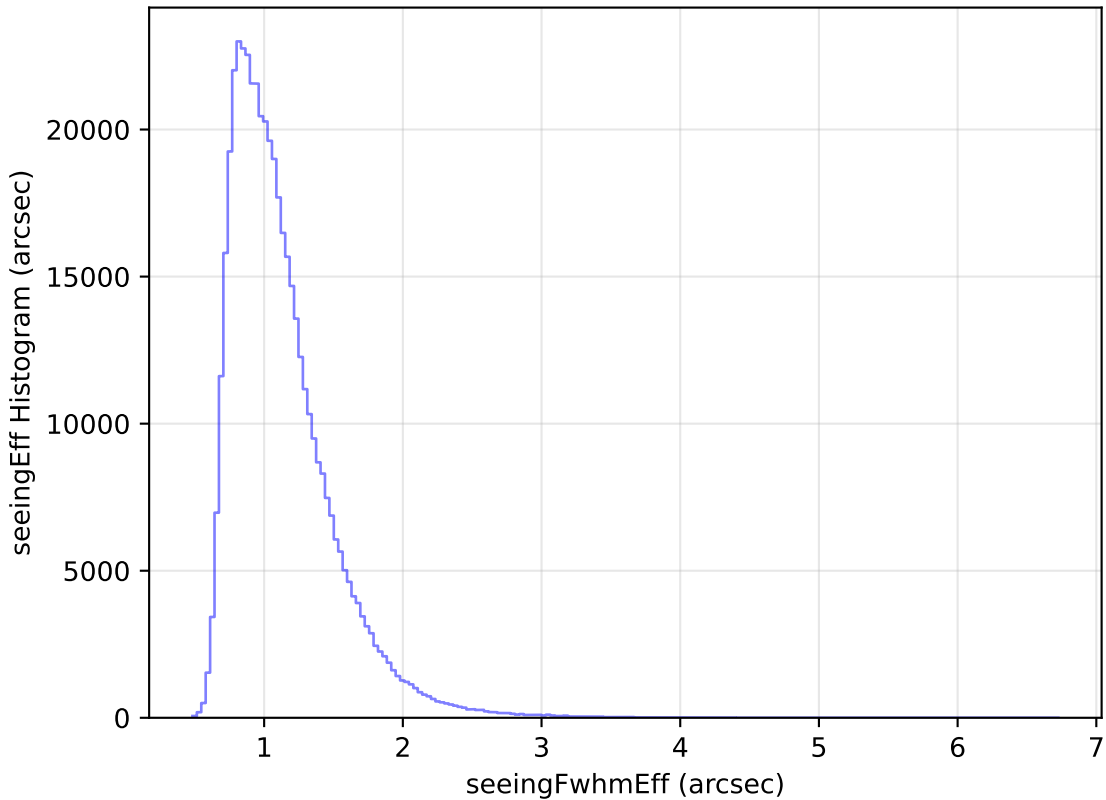
too_10_4v3.4_10yrs All sky r band: seeingEff Histogram
