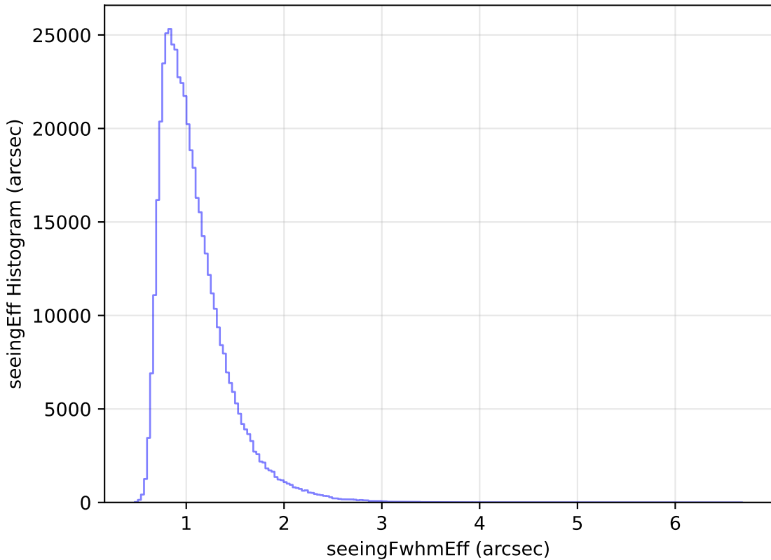
too_10_4v3.4_10yrs All sky i band: seeingEff Histogram
