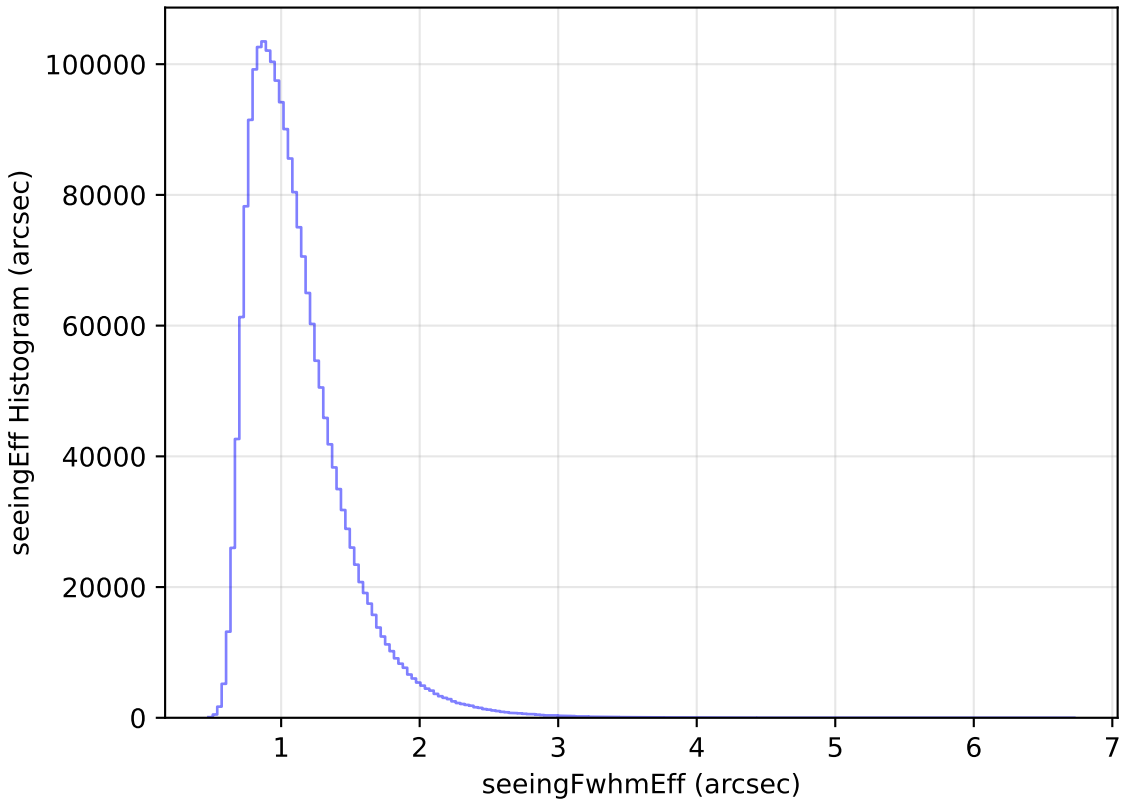
too_10_4v3.4_10yrs All sky all bands: seeingEff Histogram
