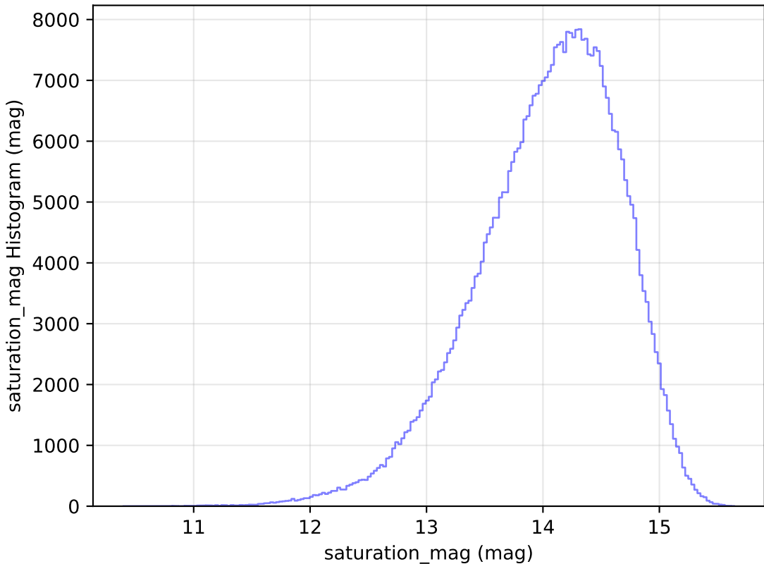
too_10_4v3.4_10yrs WFD z band: saturation_mag Histogram
