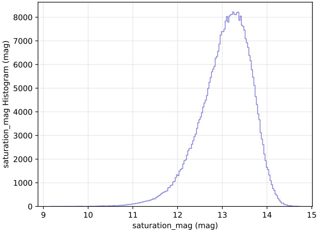
too_10_4v3.4_10yrs WFD y band: saturation_mag Histogram
