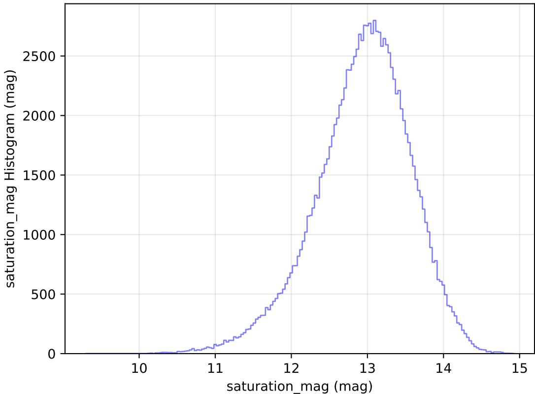
too_10_4v3.4_10yrs WFD u band: saturation_mag Histogram
