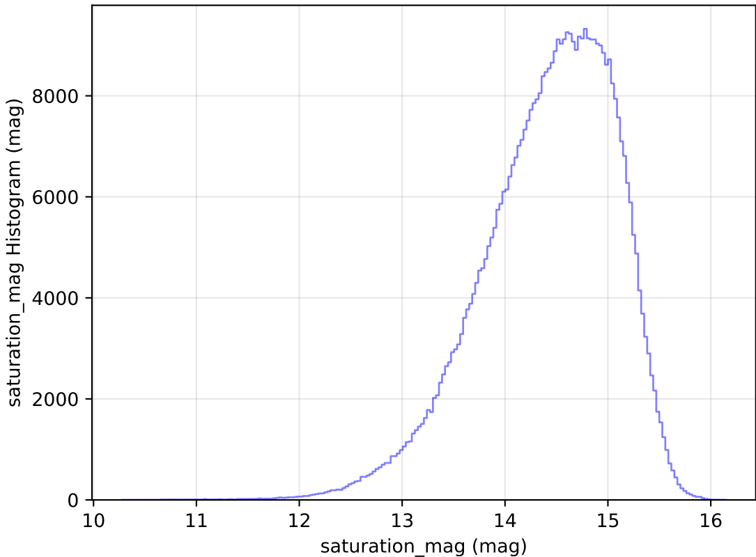
too_10_4v3.4_10yrs WFD i band: saturation_mag Histogram
