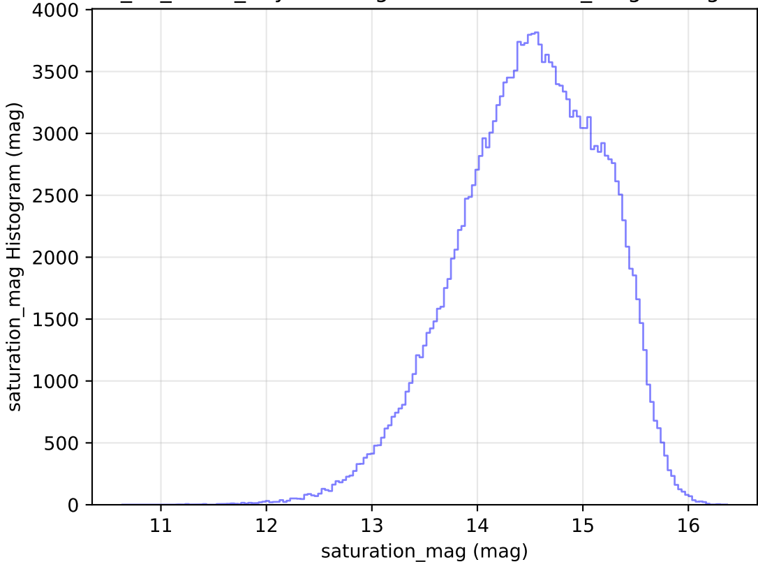
too_10_4v3.4_10yrs WFD g band: saturation_mag Histogram
