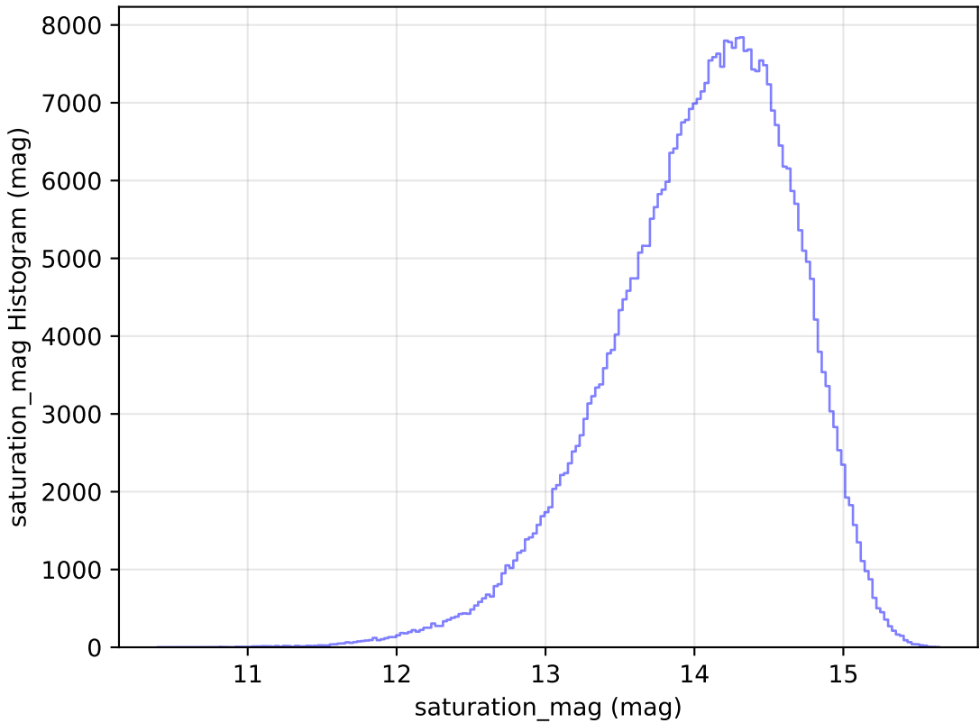
too_10_4v3.4_10yrs All sky z band: saturation_mag Histogram
