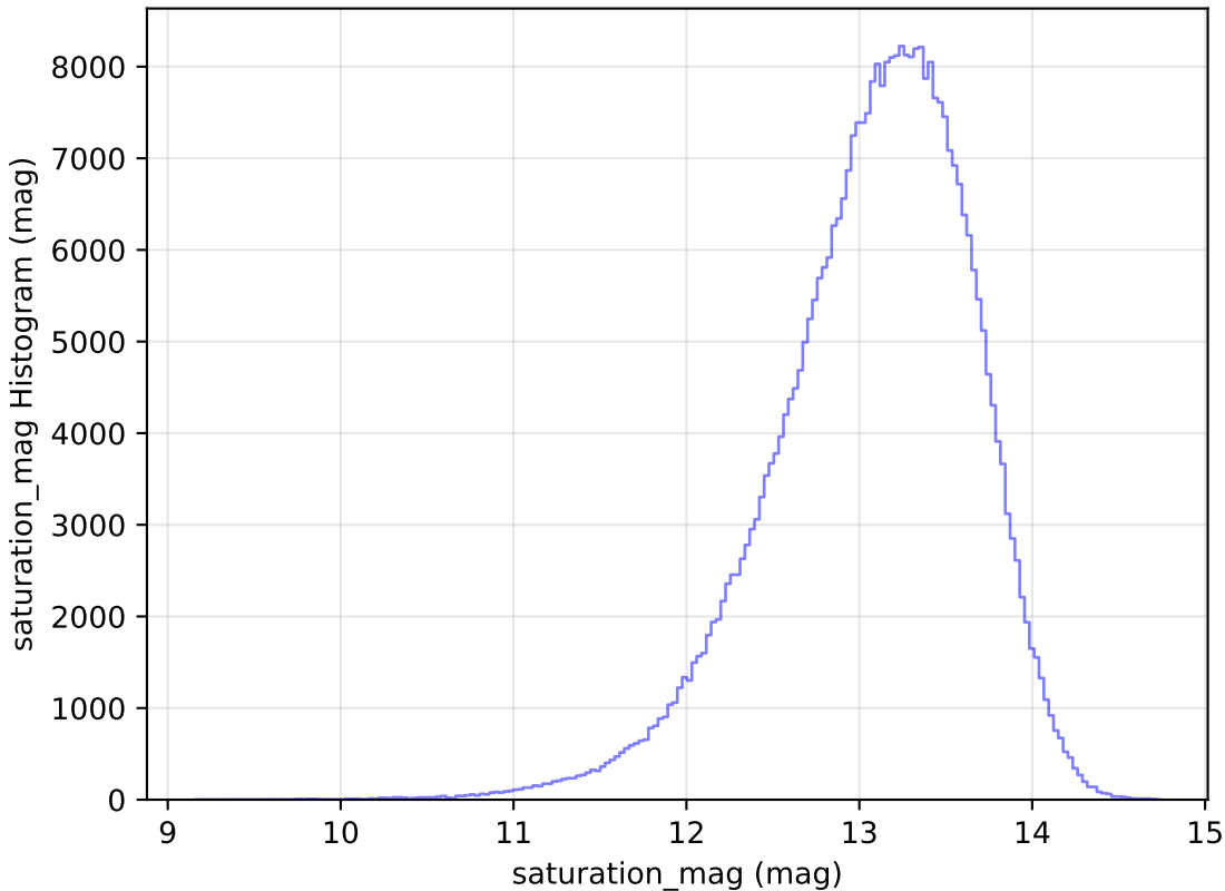
too_10_4v3.4_10yrs All sky y band: saturation_mag Histogram
